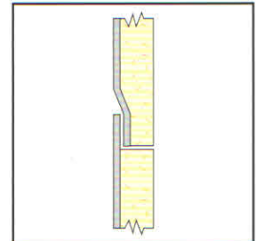
④ SOCKET & SPIGOT JOINT
