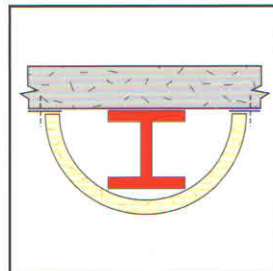
② FIX TO INTEGRAL FLANGE
